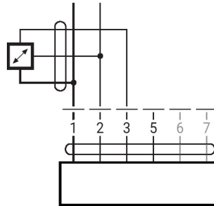
Connection with active sensor
